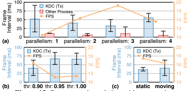
Figure 13: Parameters in real-time video streaming.
