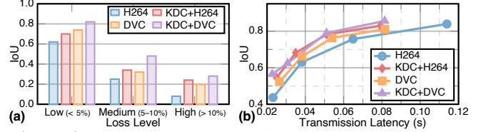
Figure 9: KDC video transmission over real Cellular networks.
