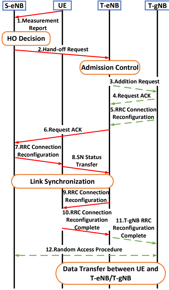
Figure 24: Hand-off procedure in the 5G NSA pattern.
