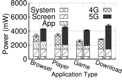
Figure 21: Energy consumption breakdown under daily app. usage.
