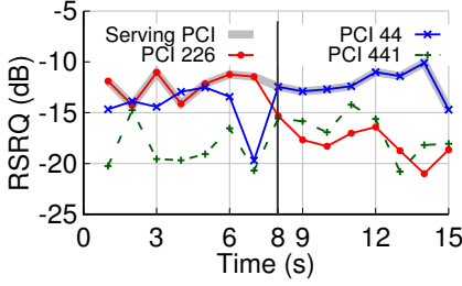
Figure 4: Signal quality evolution during hand-off (at 8s).
