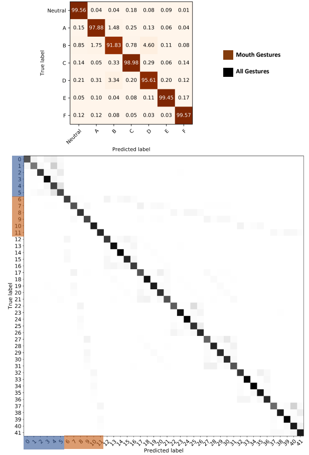
Figure 13: Confusion matrices after fine tuning the model. As we did not fine tune the classification branch for eye gestures, where therefore are not shown here. The indices can be referred to Figure 10. All results are in the units of %.
